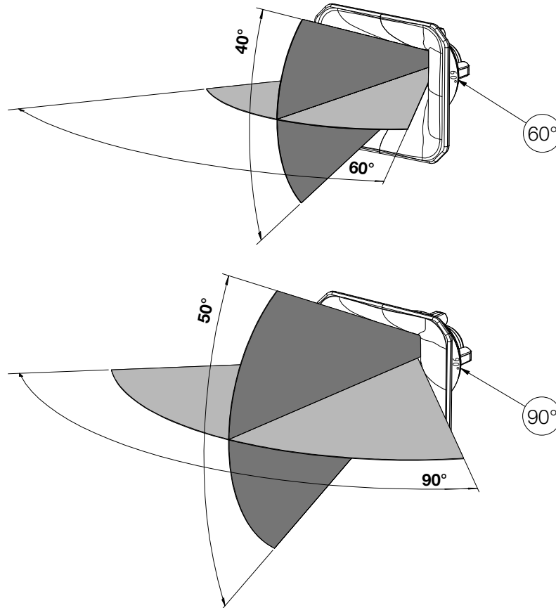
Figure 2.2.1 - Variants of the T24N horn cone
