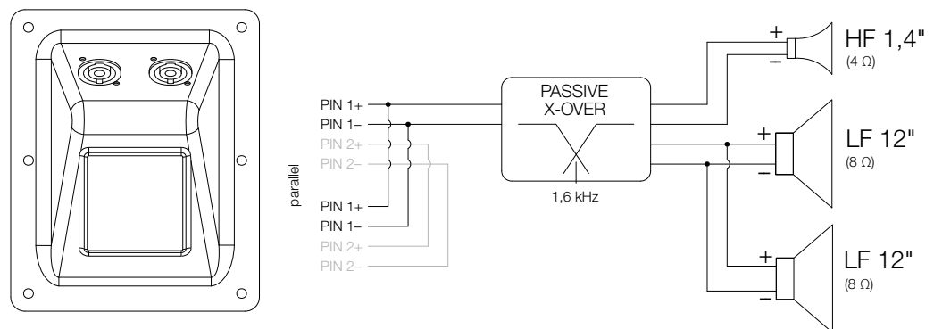
Figure 3.2.3 - Connection diagram PASSIVE
