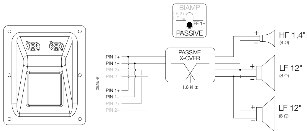
Figure 3.2.1 - Connection diagram PASSIVE switchable
