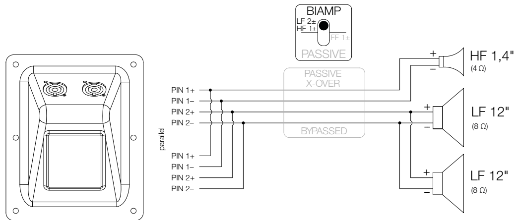
Figure 3.2.2 - Connection diagram BIAMP switchable
