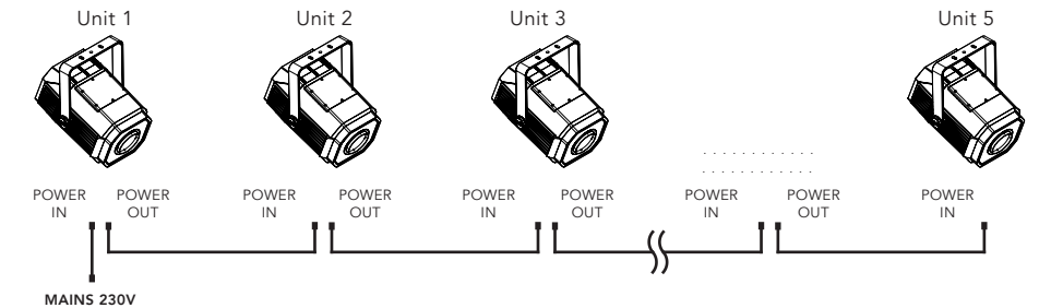
Fig. 04 - Example configuration (Output at 230 V)
