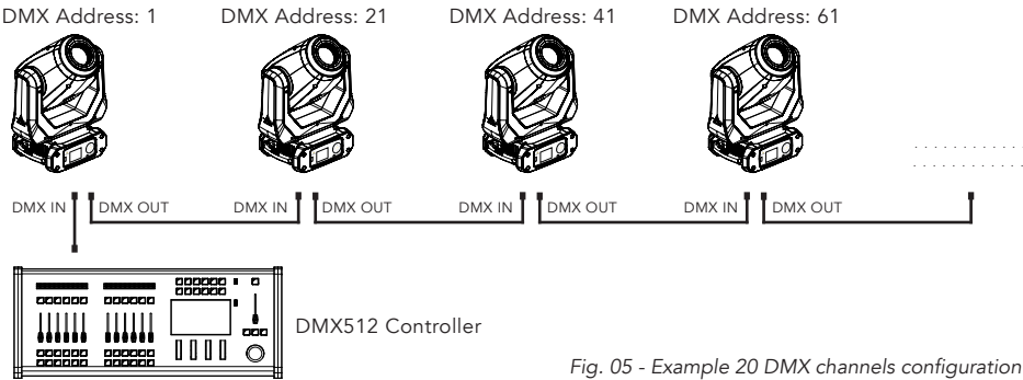
Fig. 05 - Example 20 DMX channels configuration
