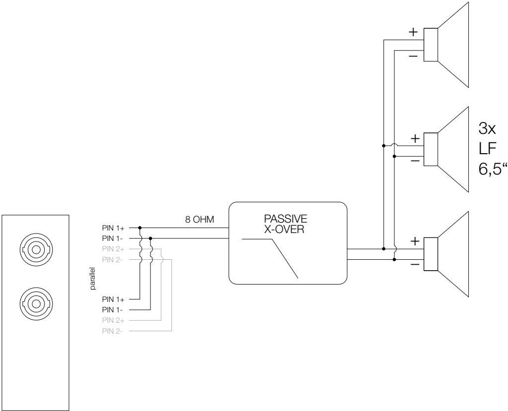
Figure 3.2 - Connection diagram
